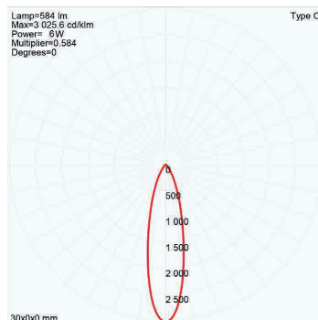
25° FWHM TIR
