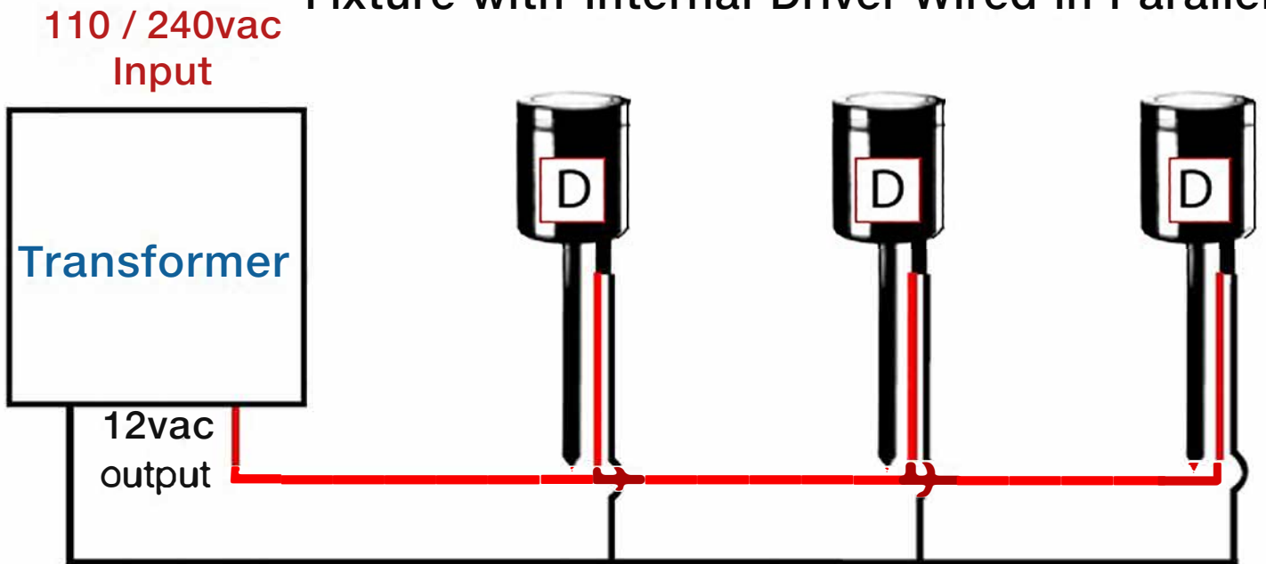
Fixture with Internal Driver Wired in Parallel
