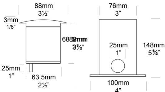
Floor Canister (supplied with luminaire)
