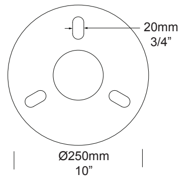
Flange Mount
