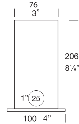
Floor Canister 200
