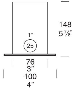
Floor Lite Canister
