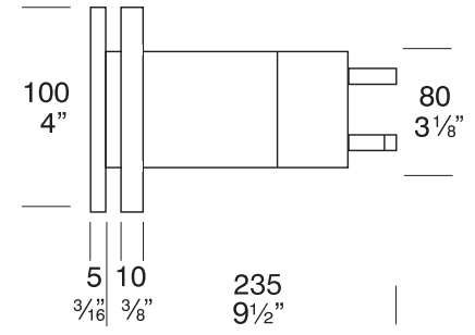
Pool Canister
