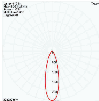
40° FWHM TIR
