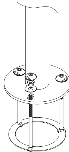
Flange Mount
