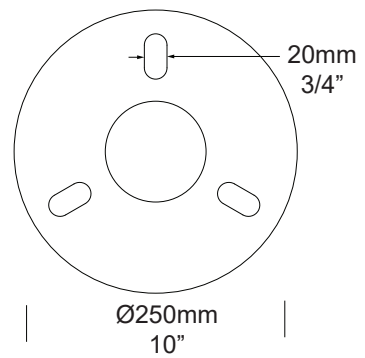
Flange Mount
