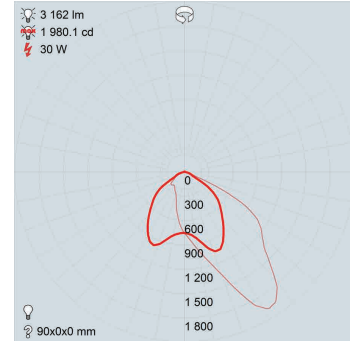
TYPE 4 OPTIC
