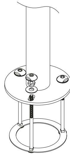
Flange Mount
